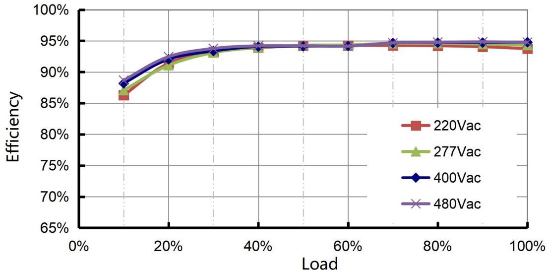
Efficiency vs. Load (C18A)
