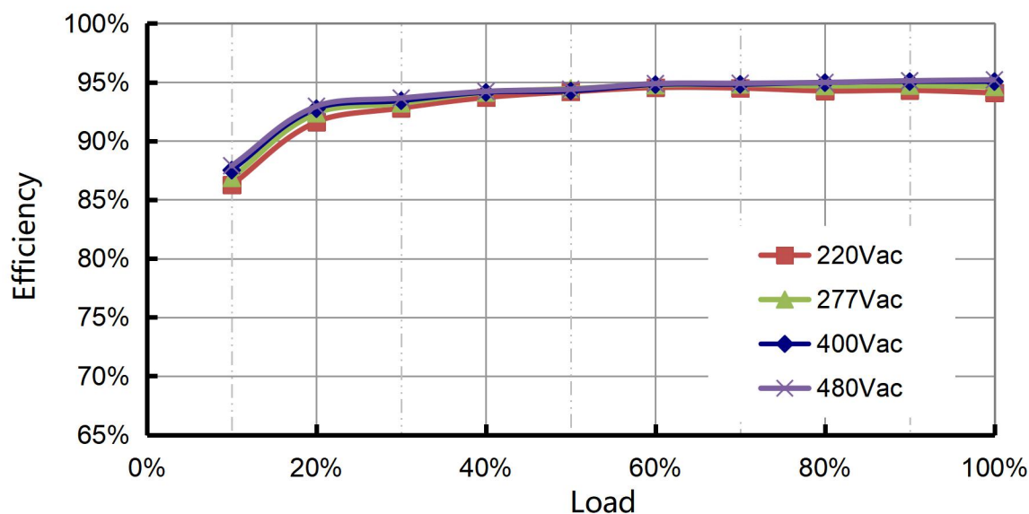
Efficiency vs. Load (C600)
