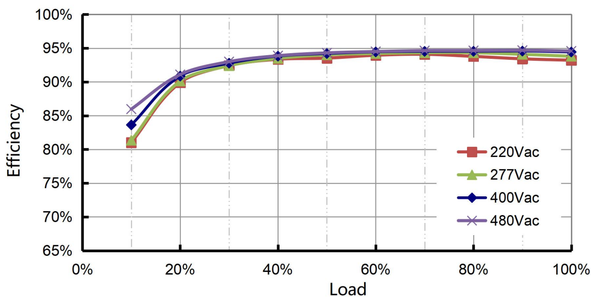
Efficiency vs. Load (C860)
